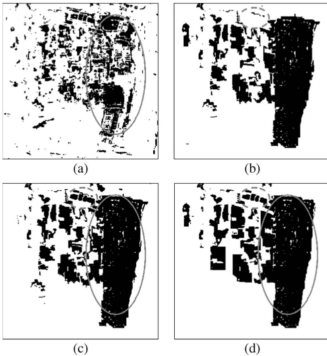
Fig. 3. Details of the change-detection maps obtained with (a) the standard pixel-based strategy, (b) the single-level parcel-based strategy applied at level 4, and (c) the proposed technique involving levels from pixel one to level 4. (d) Reference map (changed pixels appear in black, while unchanged pixels appear in white).
