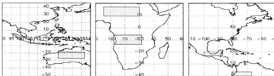
Figure 2. Geographical areas considered for evaluating the effectiveness of the proposed methods (the selected areas are within the rectangles).
