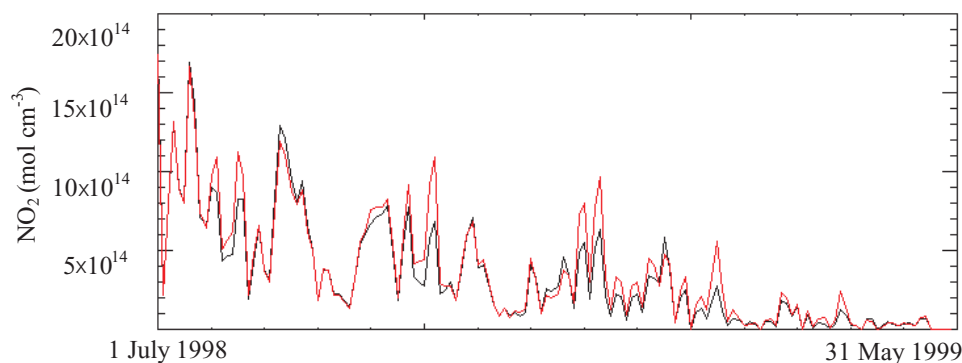
Figure 4. Amount of \text{NO}_2 emissions produced by biomass burning versus the data: values estimated with the linear approach (red line); reference values (black line) (Africa Coast region).
