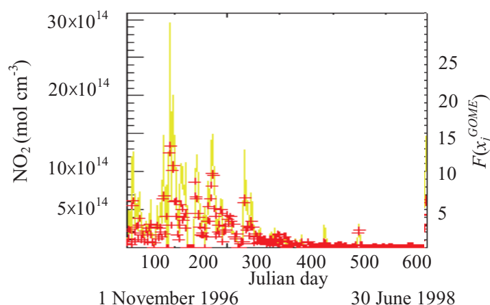
Figure 3. Abnormal amounts of \text{NO}_2 present in the troposphere versus the Julian day. The values F(x_j^{GOME}) are also reported (see red marks) (Africa Coast region).
